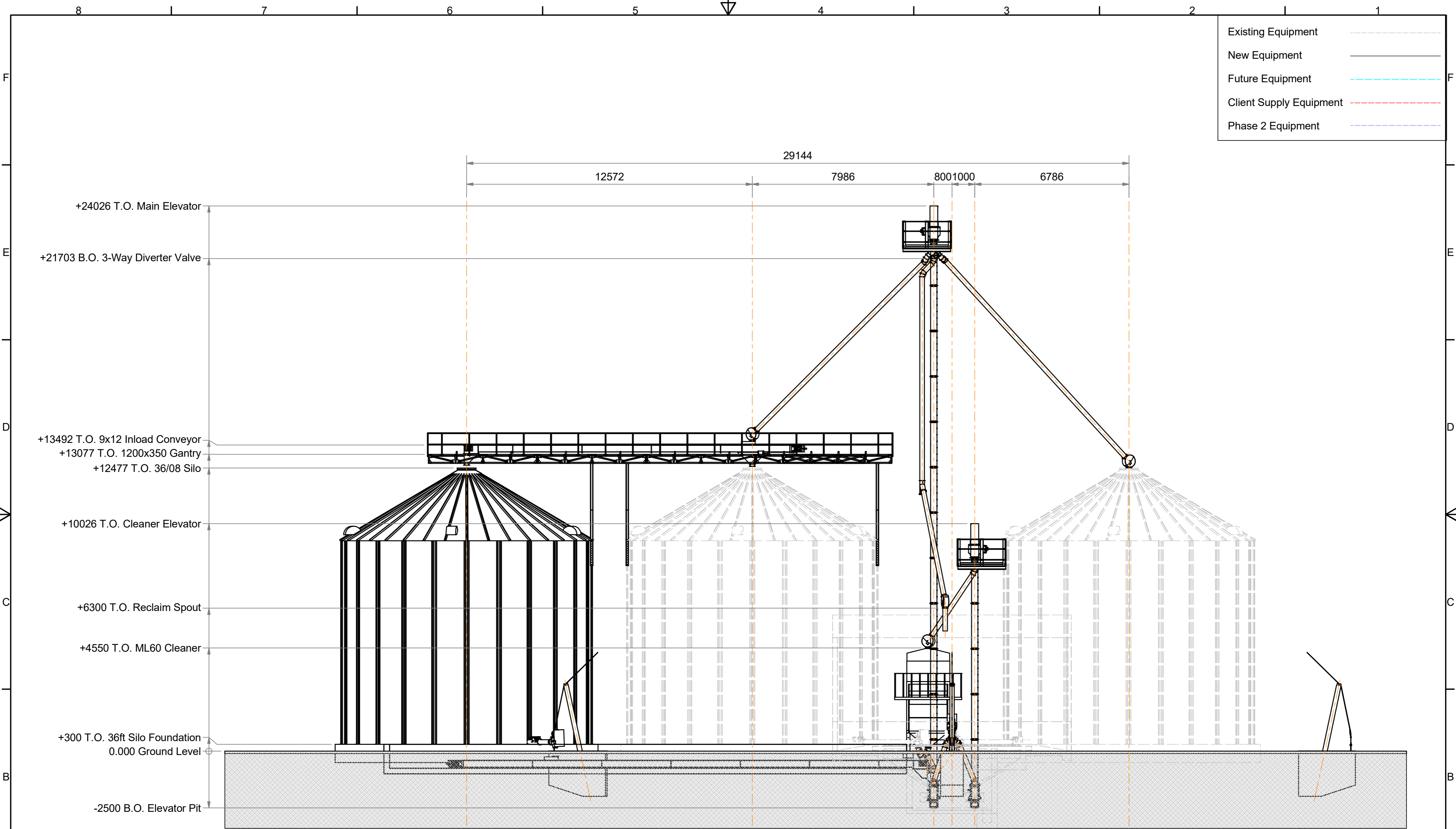
Front View Scale 1 : 110
