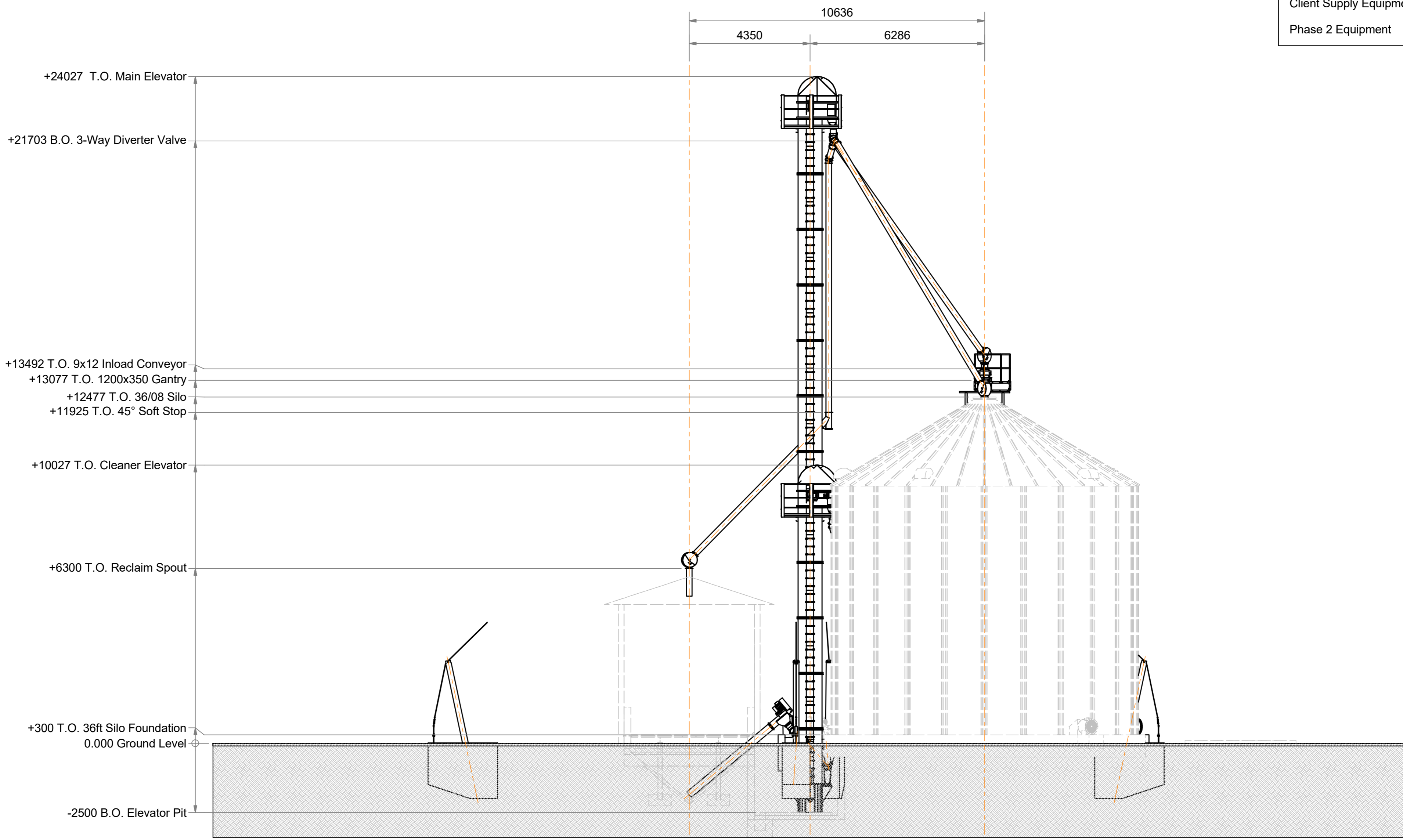
Side View Scale 1 : 100
