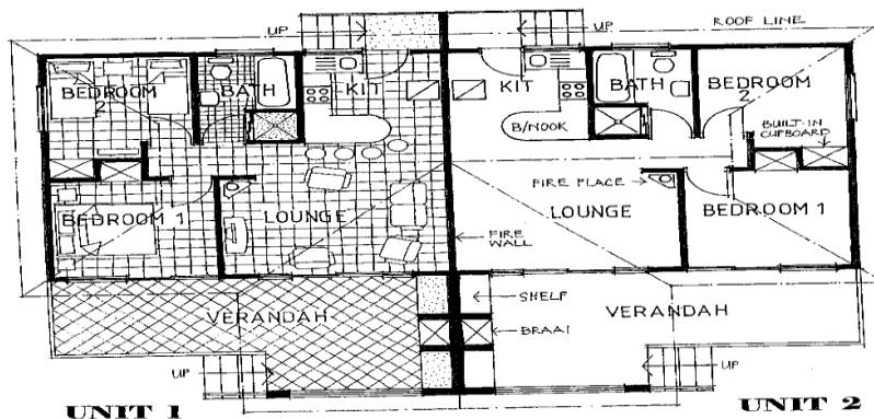
PLAN LAYOUT
